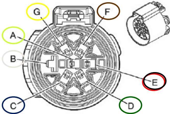
Truck-side Trailer Tow Wiring Harness
