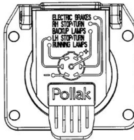
7-Way U.S.C.A.R. Trailer Plug
